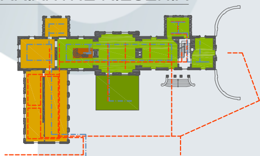
VARIANT 1. 1:200
